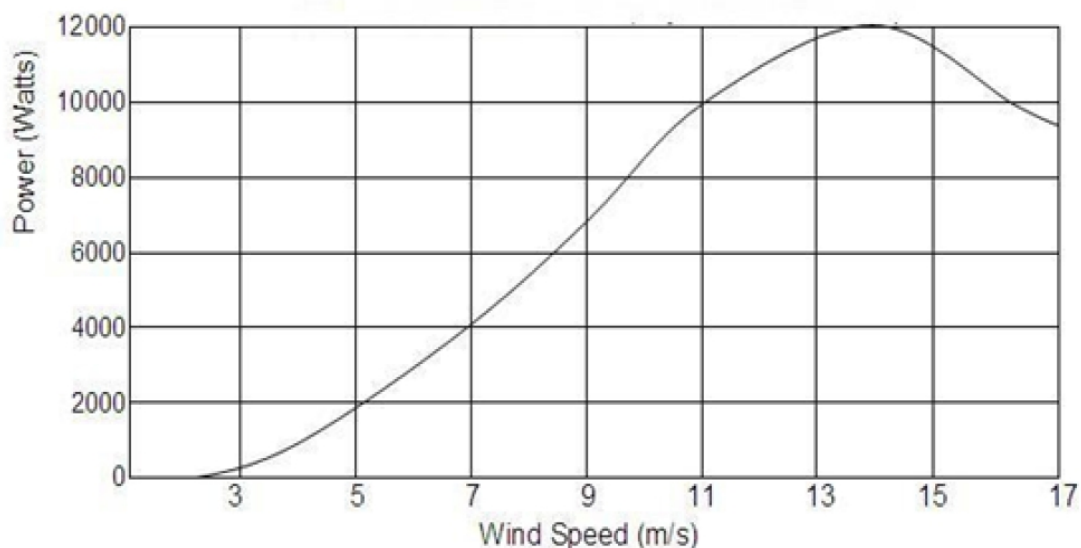
CWE-FRE-10KW Power Curve
